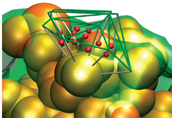
Figure 2. Visualization of a portion of the boundary layer scatterers. The green lines depict a portion of the tessellated surface generated using atomic radii (+3 Å). An inner surface (transparent green surface) was generated by dropping line segments (white lines) 3 Å in the direction opposite the surface normals at each vertex. A scattering center (red) was located at the center of each voxel at \mathbf{y}_k defined by the outer and inner triangular patches. The orange spheres correspond to heavy atoms of the molecule. The scattering from each voxel is represented as a sphere of uniform density and radius r_k , corresponding to the voxel's volume.
