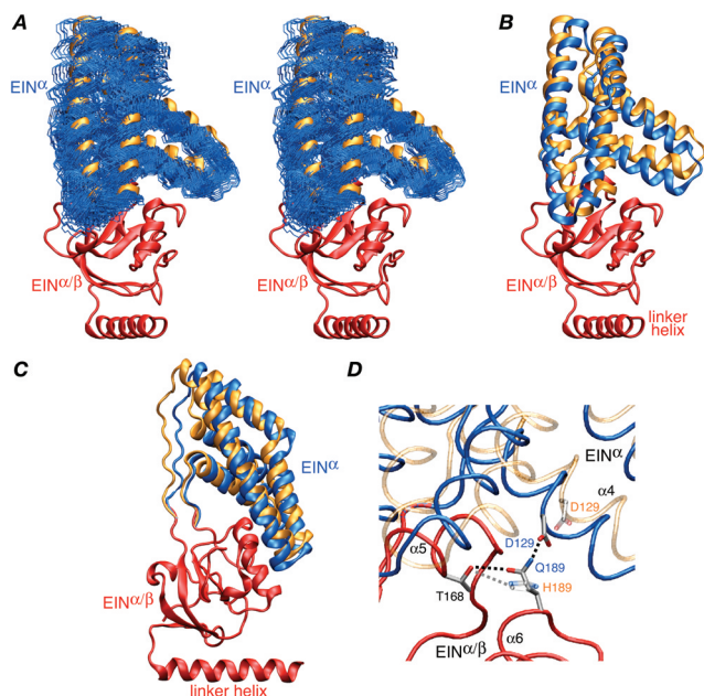
Figure 3. Structure of the EIN domain in the EI(H189Q) dimer. (A) Stereoview of the final 92 simulated annealing structures (calculated with random noise added to the RDCs) best-fitted to the EIN \alpha\beta subdomain (red ribbon), showing the precision with which the orientation of the EIN \alpha subdomain (backbone atoms in blue) relative to the EIN \alpha\beta subdomain has been determined. The location of the EIN \alpha subdomain in wild-type EI ^9 is shown as a gold ribbon. (B,C) Two views of the EIN domain with the EIN \alpha\beta subdomain superimposed (red) and the EIN \alpha subdomains of the restrained regularized mean structures of the EI(H189Q) mutant and wild-type EI ^9 in blue and gold, respectively. (D) Detail depicting the EIN \alpha /EIN \alpha\beta interface and the hydrogen-bonding interactions involving residues 189 (Gln in the mutant and His in the wild-type). The backbone of the EIN \alpha\beta subdomain of the mutant and wild-type is superimposed (red tube), and the backbone of the EIN \alpha subdomain is shown as blue and transparent gold tubes for the mutant and wild-type, respectively. The side chains of Thr168, His189/Gln189, and Asp129 are displayed, with the mutant opaque and the wild-type transparent; the dashed lines indicate hydrogen-bonding interactions.
