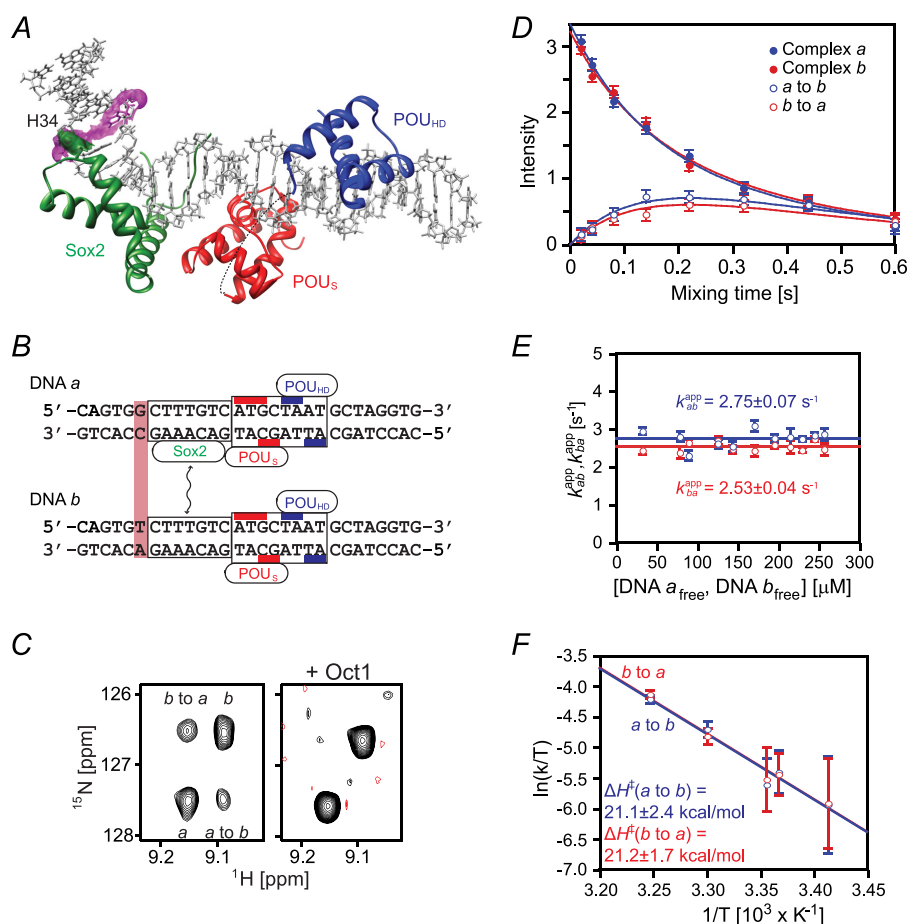
FIGURE 4. Kinetics of intermolecular translocation of Sox2 between specific DNA complexes. A , ribbon diagram of the NMR structure (Protein Data Bank code 1O4X) (23) of the Sox2-Oct1-Hoxb1-DNA ternary complex with Sox2 in green, and the POU S and POU HD domains of Oct1 in red and blue, respectively; the 29-mer DNA is shown in an all heavy atom representation. The intermolecular exchange rates for Sox2 were determined by monitoring the auto and exchange 1 H/ 15 N cross-peaks of His 34 , whose atoms are displayed as green spheres. The purple mesh identifies the base pair changed between DNA a and DNA b. B , sequences of Hoxb1 DNA fragments, DNA a and DNA b, differing by 1 base pair (light purple box). The boxes represent the Sox2 and Oct1 DNA recognition sites (with the bases contacted by the POU S and POU HD domains indicated by the red and blue bars, respectively). C , example of z-exchange data for His 34 seen in the 1 H- 15 N TROSY-based z-exchange spectrum (27) at a mixing time of 220 ms, 30 °C, and 150 mM NaCl for the Sox2-Hoxb1-DNA binary (left) and Oct1-Sox2-Hoxb1-DNA ternary complexes (right). The concentrations of 2 H/ 15 N-labeled Sox2, DNA a, DNA b, and Oct1 (at natural isotopic abundance) are 0.55, 0.35, 0.35, and 0.7 mM, respectively. D , time dependence of auto (closed circles) and exchange (open circles) cross-peak intensities at 30 °C and 150 mM NaCl together with the best fit curves (solid lines). The concentrations of 2 H/ 15 N-labeled Sox2, DNA a and DNA b are 0.55, 0.35, and 0.35 mM, respectively. E , apparent intermolecular exchange rates as a function of free DNA concentration. The rates are independent of free DNA concentration, indicating that the rate-limiting step is governed by dissociation of Sox2 from the DNA. F , Eyring plots of the apparent intermolecular exchange rates at 20, 24, 25, 30, and 35 °C and 150 mM NaCl. Linear fits for the exchange rates k_{ab}^{app} and k_{ba}^{app} are shown as blue and red lines, respectively. Thermodynamic parameters derived from the data are shown in Table 1. Error bars, S.D.
