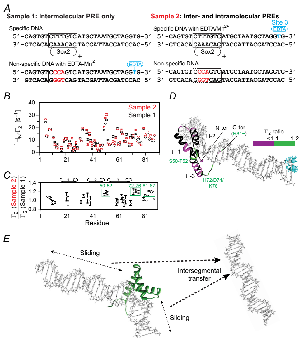
FIGURE 6. Intramolecular versus intermolecular translocation of Sox2 in the specific Sox2-Hoxb1-DNA binary complex. A, the samples comprise an equimixture of specific and nonspecific 29-bp DNA duplexes. In sample 1, the specific DNA duplex is unlabeled, and the nonspecific DNA duplex bears the paramagnetic label. In sample 2, the specific DNA duplex is paramagnetically labeled at site 3 (cf. Fig. 5A), and the nonspecific DNA duplex is unlabeled. The PRE effects observed for sample 1 arise entirely from intermolecular translocation, whereas those for sample 2 arise from both intra- and intermolecular translocation processes. The concentrations of Sox2, specific DNA, and nonspecific DNA are 0.40, 0.45, and 0.45 mM, respectively. B, PRE profiles at 150 mM NaCl from samples 1 and 2 shown as black and red circles, respectively (error bars, S.D.). C, ratio of PRE rates for sample 2 to sample 1 for residues with 1 H N -Γ 2 rates of >10 s -1 . For Γ 2 (sample 2)/Γ 2 (sample 1) ~ 1, the PRE effects arise predominantly from intermolecular translocation; Γ 2 (sample 2)/Γ 2 (sample 1) ratios larger than 1 are indicative of contributions from both intra- and intermolecular translocation, where the contribution from the latter is provided by the PRE profiles observed for sample 1. D, mapping of Γ 2 ratios (color scale indicated on the right) onto the structure of the specific Sox2-DNA complex (23). E, schematic of intramolecular (sliding) and intermolecular (intersegment transfer) translocation events involving Sox2 bound specifically to DNA. Because bulk intersegment transfer of Sox2 between specific sites involves complete dissociation of Sox2 into free solution, followed by reassociation, the sparsely populated states arising from intermolecular translocation from the specific duplex to a nonspecific duplex and back again sampled by PRE must involve an initial sliding event from the specific site to an adjacent nonspecific site, followed by direct intersegment transfer to the nonspecific duplex and then back to the specific duplex.
