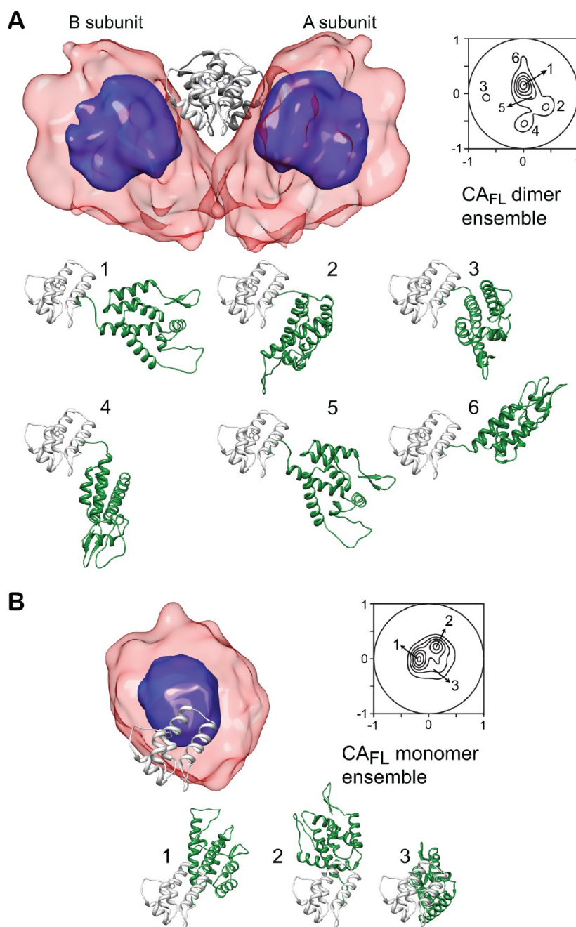
Figure 6. Structural ensembles calculated for the wild-type capsid ( CA_{FL} ) dimer (A) and monomer (B). The overall distribution of the N-terminal domain relative to the C-terminal domain (light and dark gray ribbons) is displayed as a reweighted atomic probability plotted at 50% (blue) and 10% (transparent red) of maximum. Also shown are projection contour maps that display the distribution of the position of the centroid of the N-terminal domain relative to the C-terminal domain (see Materials and Methods). The dimer and monomer ensembles are characterized by six and three main clusters, respectively. Representative structures from each cluster are shown as ribbon diagrams with a single C-terminal domain subunit in light gray and the N-terminal domain in green. The orientation of the displayed C-terminal domain for the dimer and monomer clusters is the same as that of the A subunit (light gray) shown in the top of panel A. For simplicity, only a single subunit is shown for the six dimer clusters.
