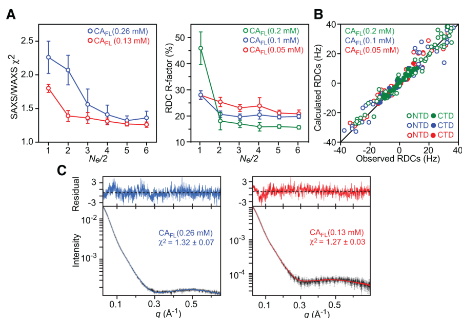
Figure 4. SAXS/WAXS and RDC-driven ensemble simulated annealing refinement of the wild-type capsid protein CA FL . Each ensemble comprises the same number of monomers and dimers (i.e., N_e/2 = N_e^{\text{dimer}} = N_e^{\text{mon}} ) weighted according to their populations at different concentrations as determined by analytical ultracentrifugation (Table 3). (A) SAXS/WAXS \chi^2 and C-terminal domain RDC R-factors as a function of ensemble size N_e/2 . Note that the RDC R-factors for the N-terminal domain show a much smaller decrease with increasing N_e (see Table 5 and Figure S1B). (B) Agreement between observed and calculated 1 D NH RDCs at three CA FL concentrations (0.2, 0.1, and 0.05 mM shown in green, blue and red, respectively). Note the smaller span of the RDCs for the C-terminal domain (filled-in circles, \sim \pm 15 Hz) compared to those for the N-terminal domain (open circles, \sim \pm 40 Hz). (C) Agreement between observed and calculated SAXS/WAXS curves. The experimental SAXS/WAXS data are shown in black with gray vertical bars equal to 1 SD, and the calculated curves are shown in blue and red for the data at CA FL concentrations of 0.26 and 0.13 mM (in subunits), respectively. The residuals, given by (I_i^{\text{calc}} - I_i^{\text{obs}})/I_i^{\text{err}} , are plotted above the curves.
